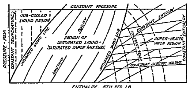
FIG. 1-4. Typical Pressure-Enthalpy Diagram for a Refrigerant.
