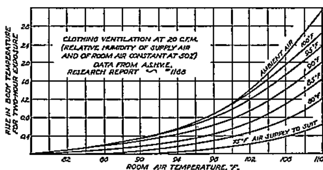
FIG. 14-4. Local Cooling by Ventilation of Clothing.
