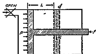
FIG. 1-1. Flow Work during Admission.
