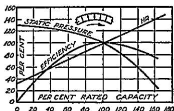
FIG. 15-5. Radial Blade Characteristics.
