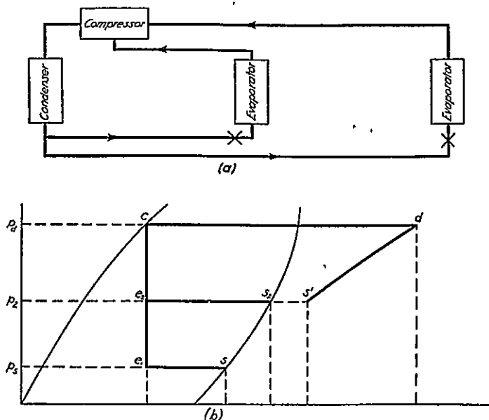
FIG. 3-12. Sectionalizing with Multi-effect Compression.
