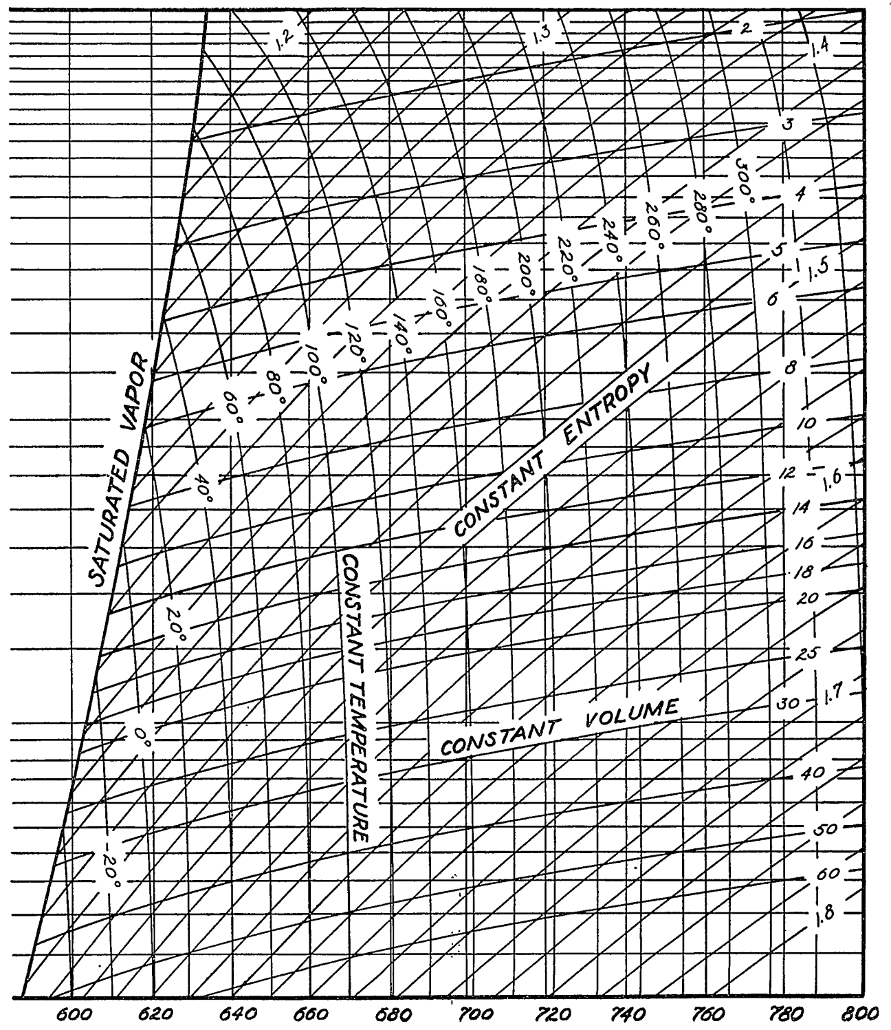
Pressure-Enthalpy Chart for Ammonia. (From data in Circular 142 of the U. S. Bureau of Standards.)
