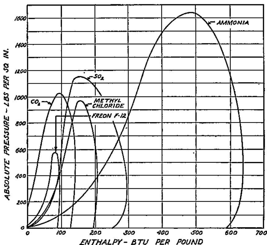
FIG. 1-3. Comparison of Refrigerants:
