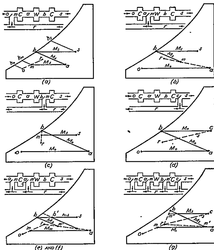
FIG. 12-15. Recirculation for Heating Season.
