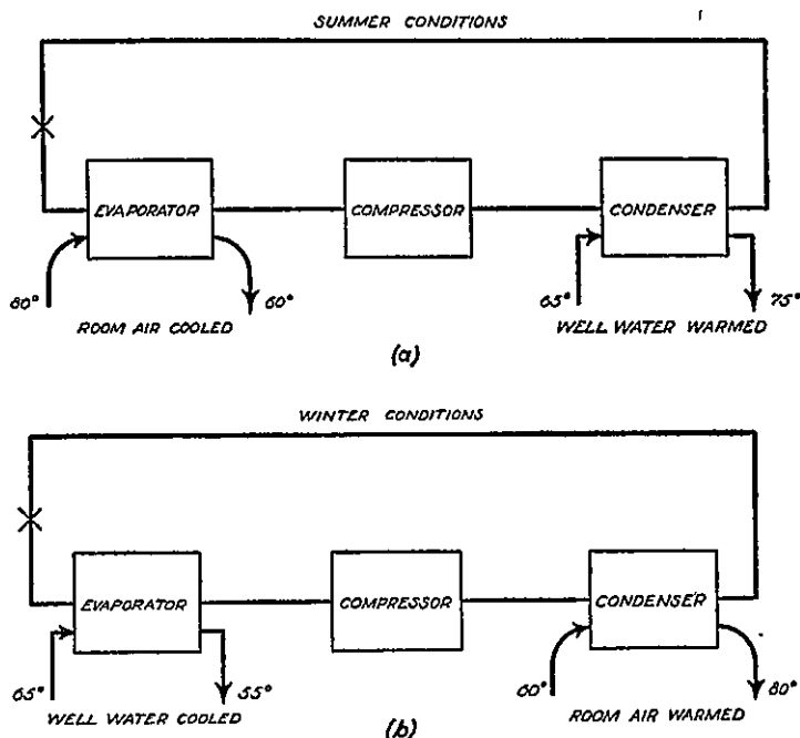
FIG. 4-8. Heat Pump Using Well Water.
