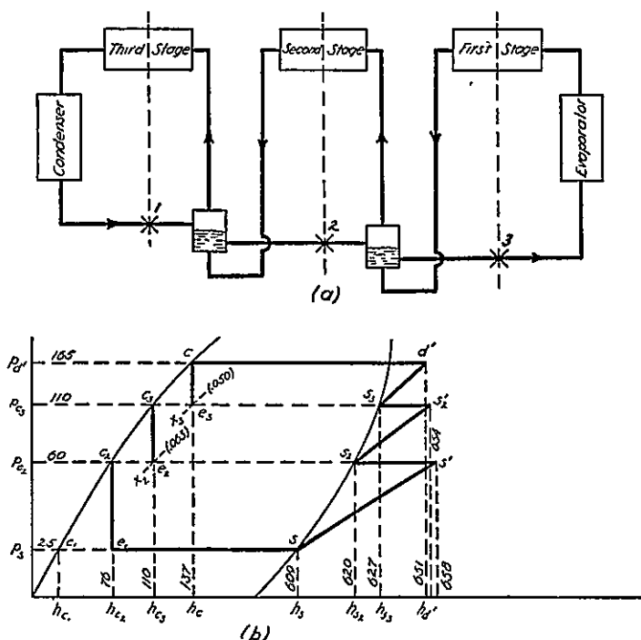
FIG. 3-5. Compound Compression with Flash Intercooling.
