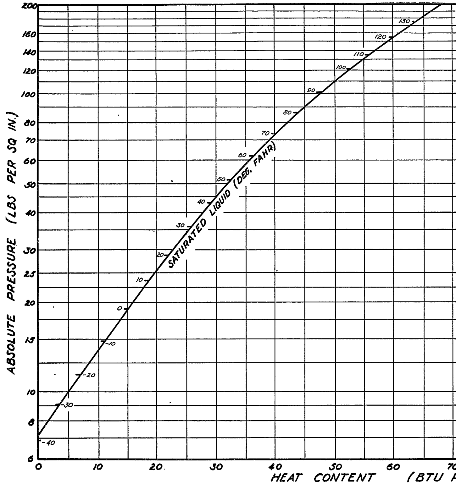
Pressure-Enthalpy Chart for Methyl Chloride.
