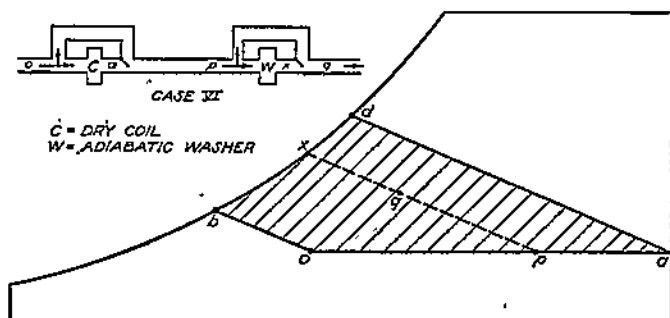
FIG. 12-3. Dry Coil Preceding Adiabatic Washer.
