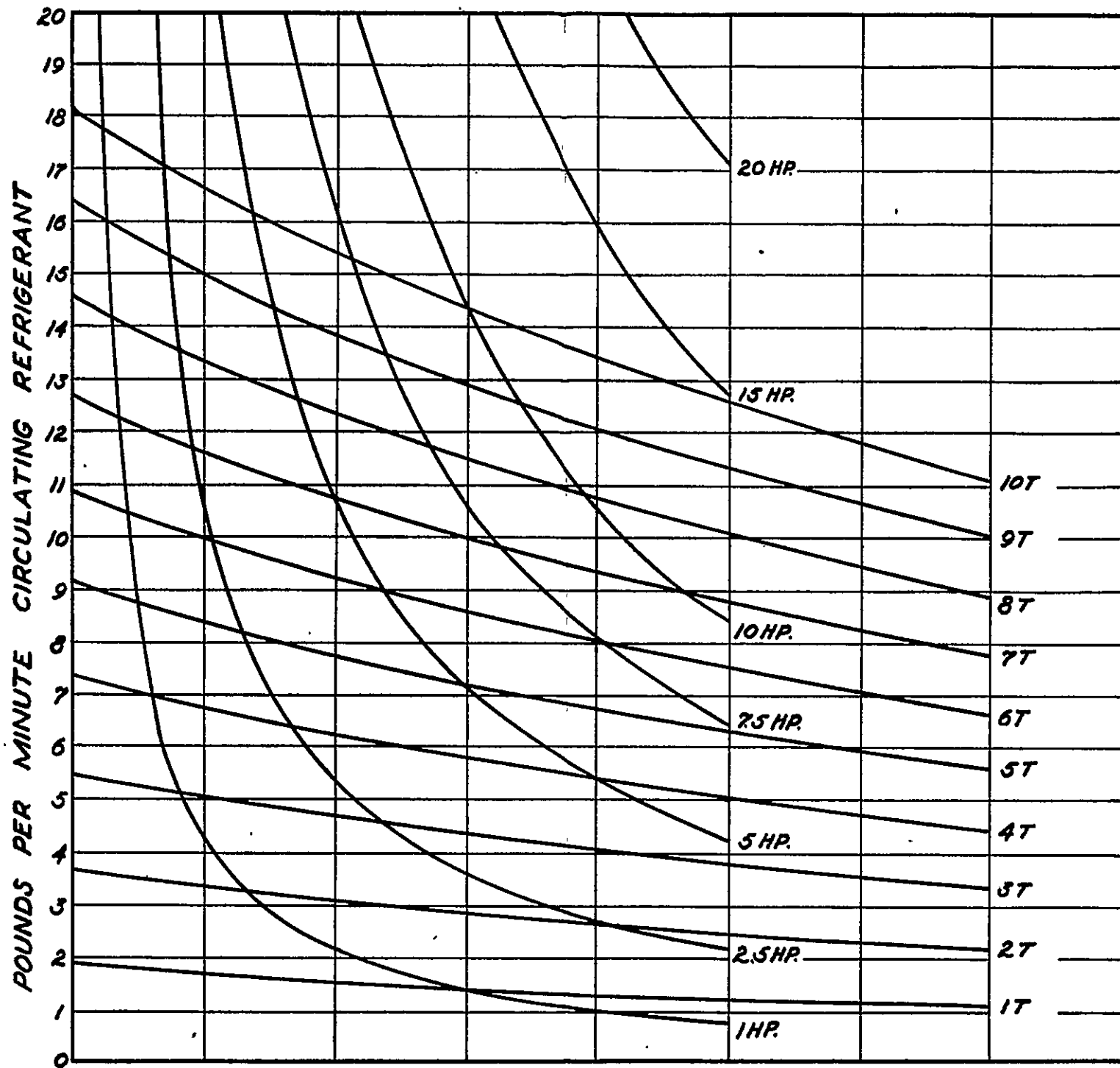
Trace Sheet for Sulfur Dioxide.
