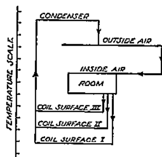
FIG. 11-4. Energy Lift Diagram.
