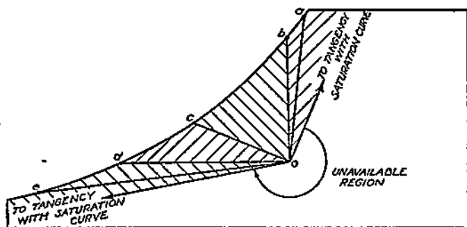
FIG. 11-14. Washer Processes; High Water-air Ratio.
