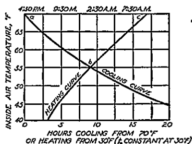
Fig. 8-4. Typical Heating and Cooling Curves.
