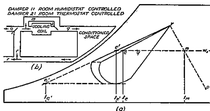
FIG. 11-2. Variable Surface Temperature (Humidity Controlled).
