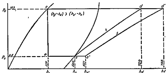
FIG. 2.5. Simple Superheating Cycle.
