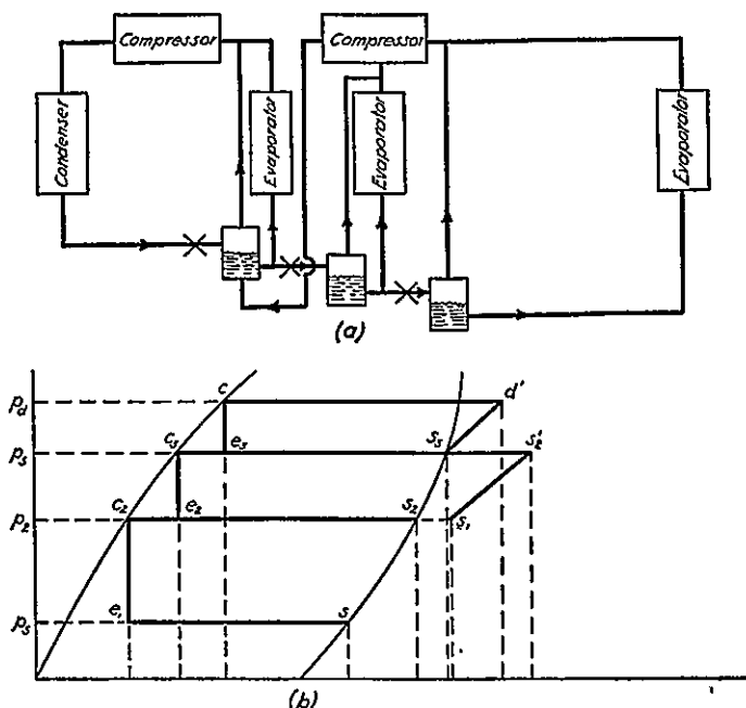
FIG. 3-14. Typical Multiple Load Cycle.
