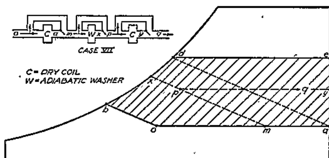
FIG. 12-4. Tempering Coil, Adiabatic Washer, and Reheat Coil.
