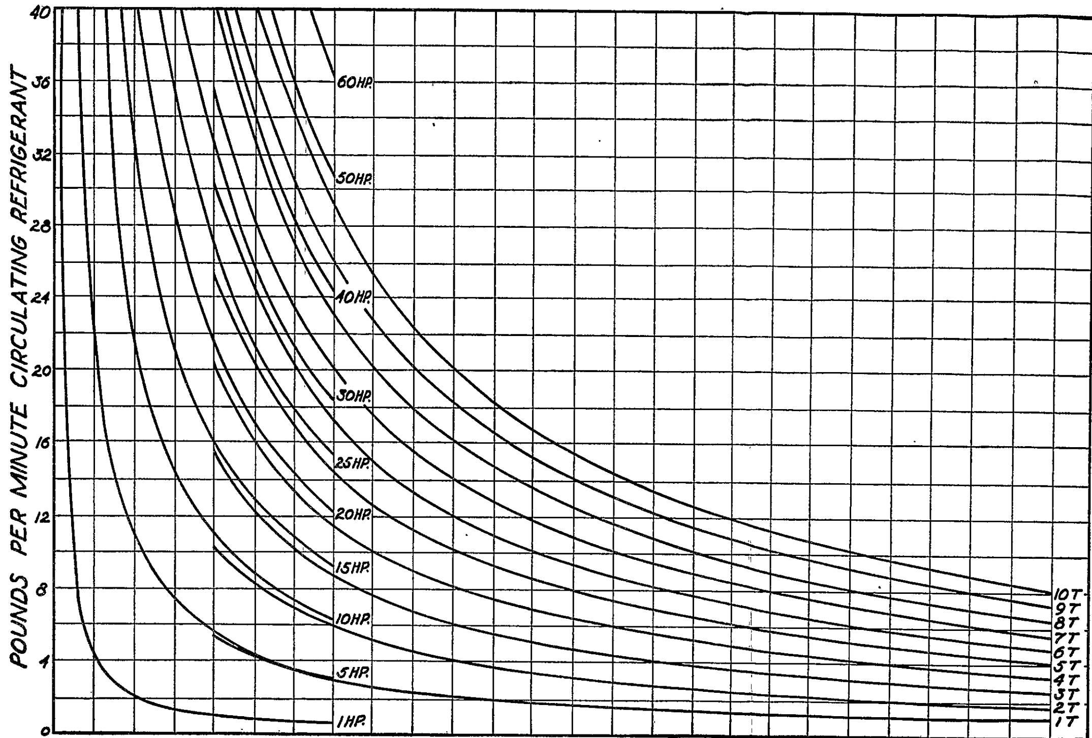
Trace Sheet for Carbon Dioxide.
