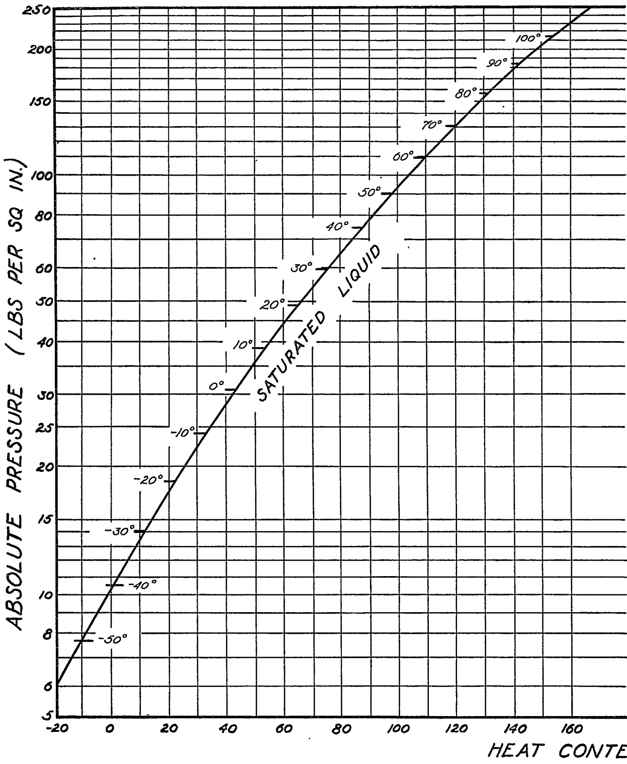
Pressure-Enthalpy Chart for Ammonia. (From data in Circular 142 of the U. S. Bureau of Standards.)
