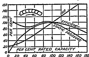
FIG. 15-3. Forward Blade Characteristics.
