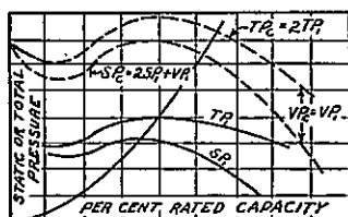
Fig. 15-8. Series Operation of Fans.
