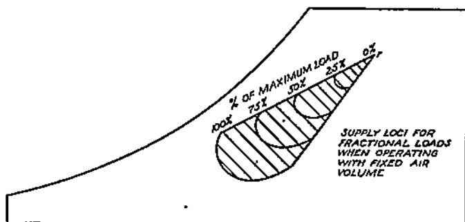
FIG. 10-3. Supply Loci for Fractional Loads.
