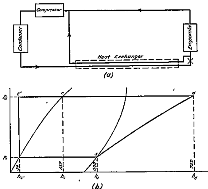
FIG. 2.7. Subcooling with Liquid Refrigerant.
