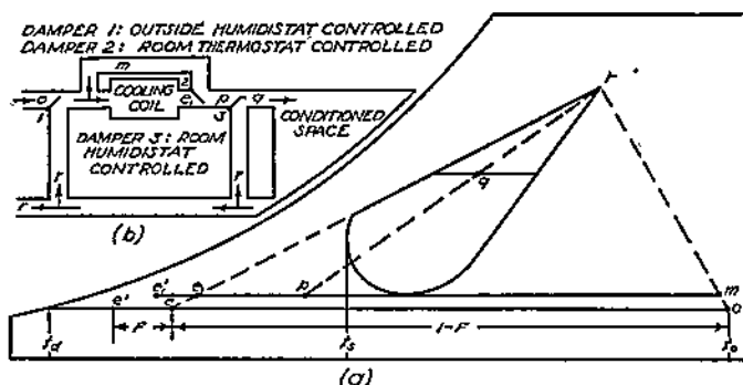
FIG. 11-1. Fixed Surface Temperature.
