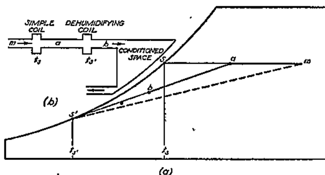
FIG. 11-9. Precooling and Dehumidifying Coils in Series.
