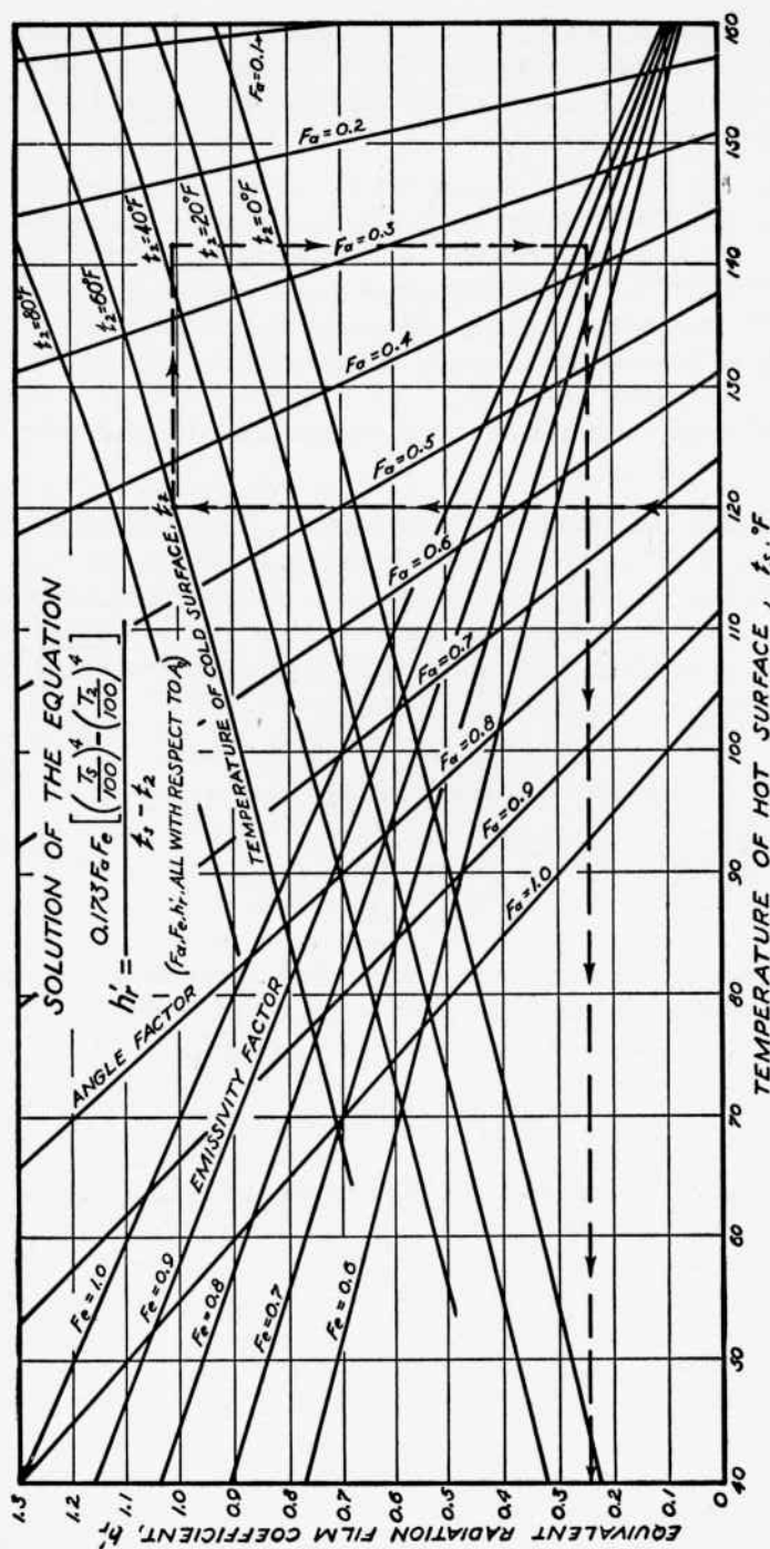
Fig. 6-4. Graphical Determination of Equivalent Radiation Coefficient.
