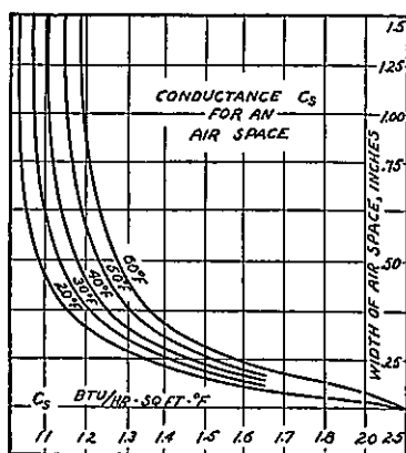
FIG. 6-3. (From tabular data in ASHVE Guide, p. 92, 1944.)
