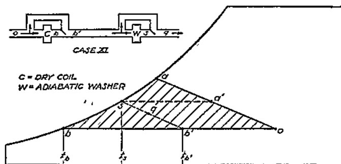
FIG. 12·7. Dry Cooling Coil and Adiabatic Washer.
