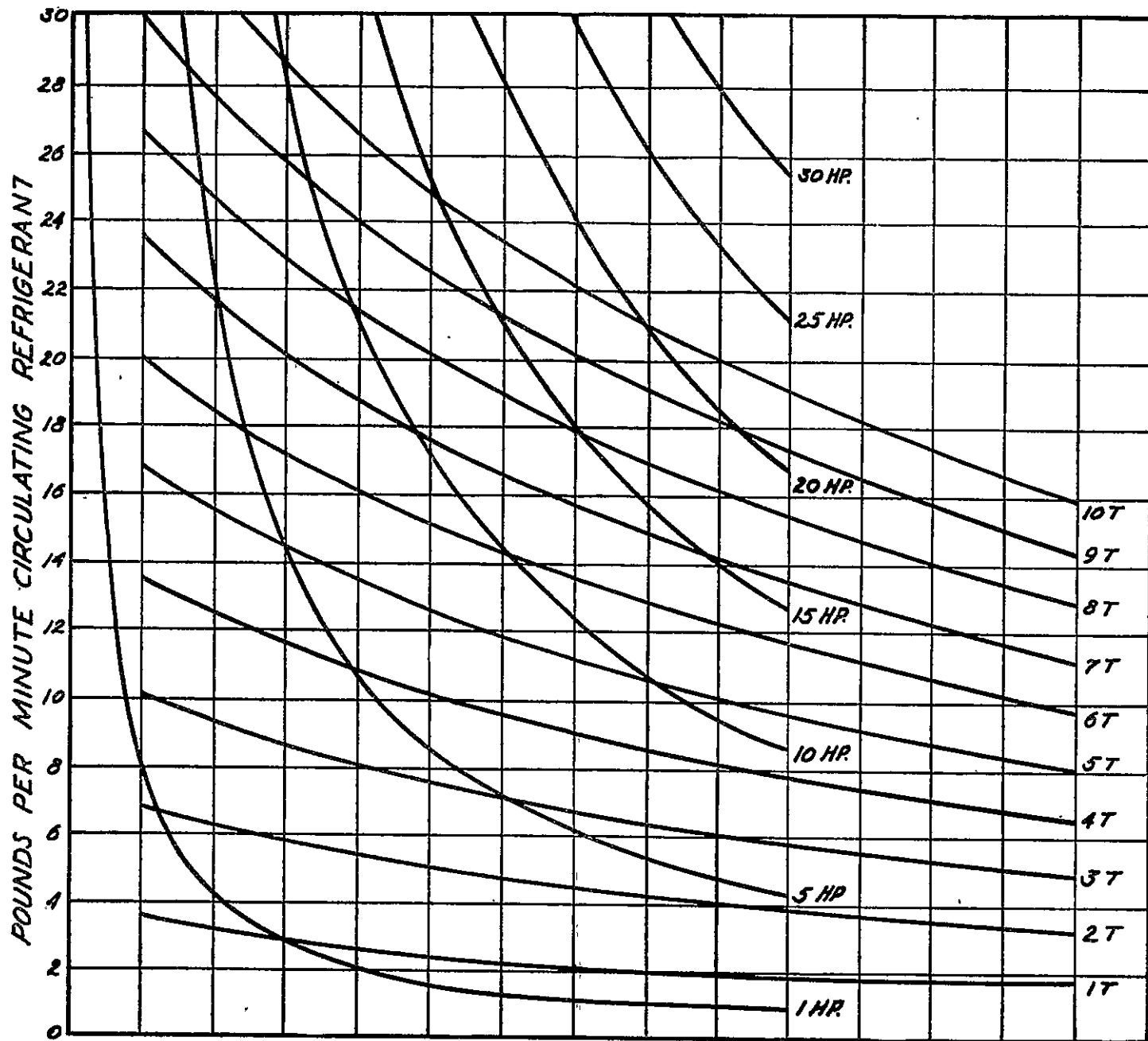
Trace Sheet for Freon-21.
