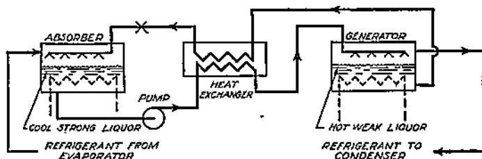
FIG. 5-1. Elements of Ideal Absorption System.
