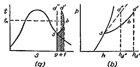
Fig. 4.3. Heat Transfer during Compression Process.
