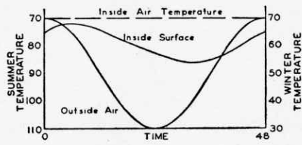
FIG. 7-4. (Upper left). Graphical Solution of Homogeneous Wall Problem. FIG. 7-5. (Lower right). Time-temperature Curve.
