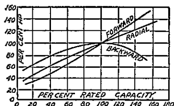
Fig. 15-6. Comparative Horsepower Curves.
