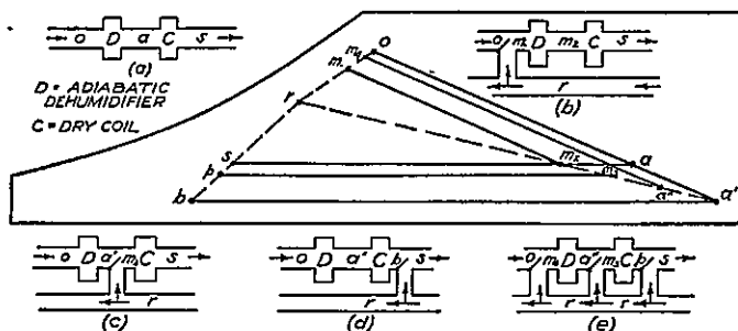
FIG. 12-16. Recirculation for Cooling Season.
