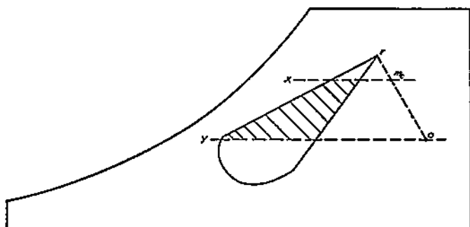
FIG. 11-5. Humidity Limitation with Simple Cooling.
