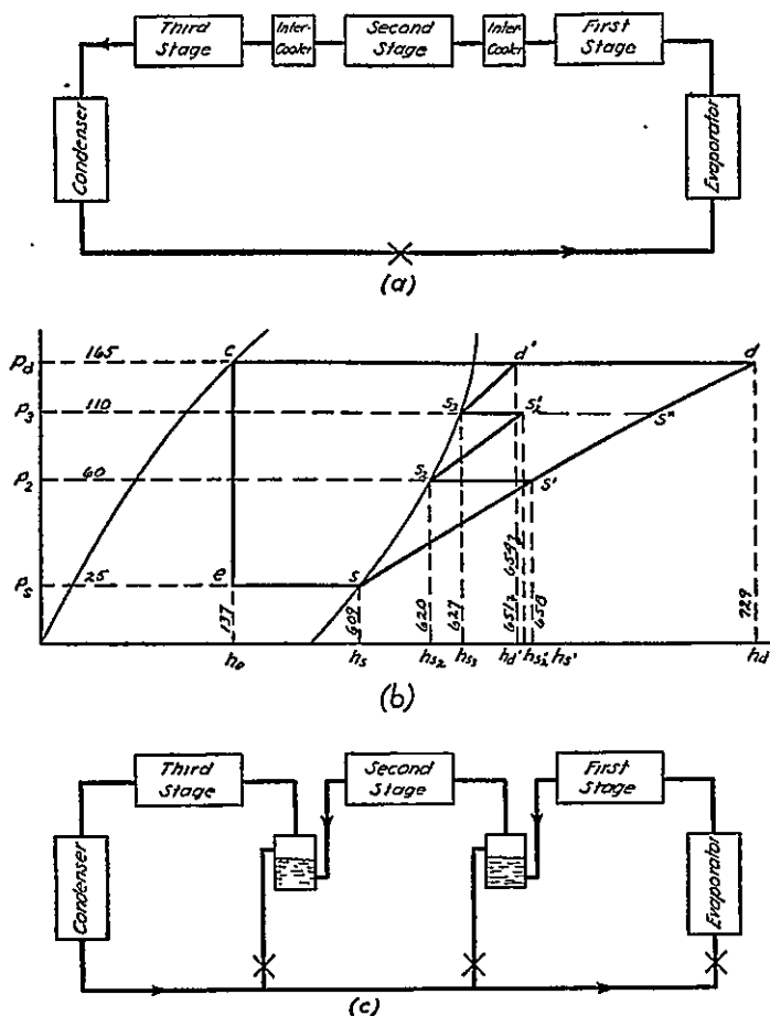
FIG. 3-3. Compound Compression Cycle.
