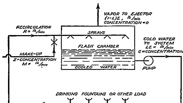
FIG. 4-6. Steam Jet Direct Water Cooling.
