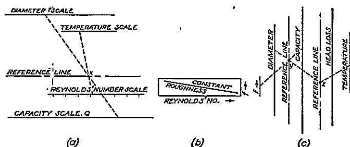
FIG. 16-1. Detail of Friction Chart Construction.
