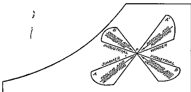
FIG. 10-4. Four Types of Supply Problems.
