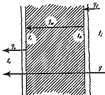
FIG. 6-2. Air-to-air Heat Transfer.
