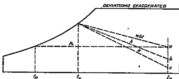
FIG. 9-4. State-point Determination.
