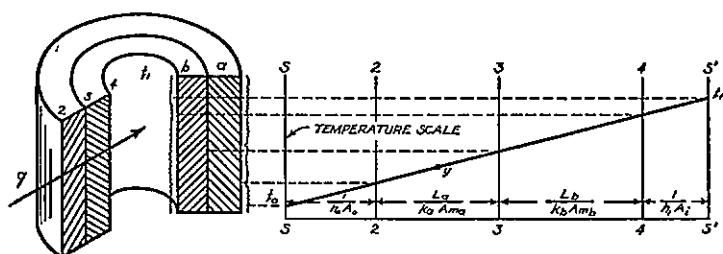
Fig. 6-5. Graphical Temperature Determination:
