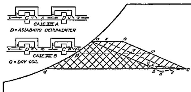
FIG. 12-9. Dry Cooling Coil and Adiabatic Dehumidifier.
