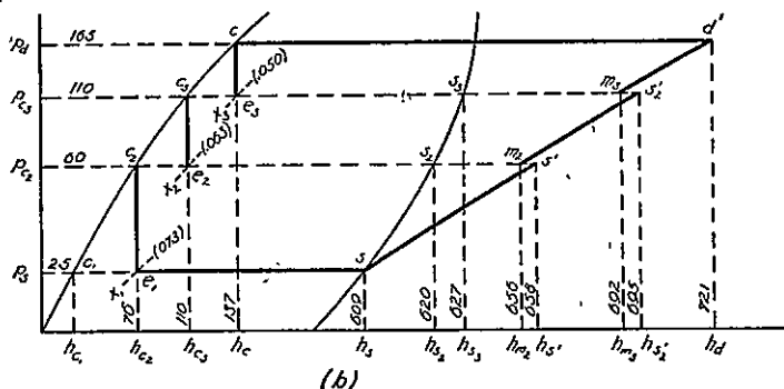
FIG. 3.4. Compound Cycle, Multiple Expansion Valves, No Intercooling.
