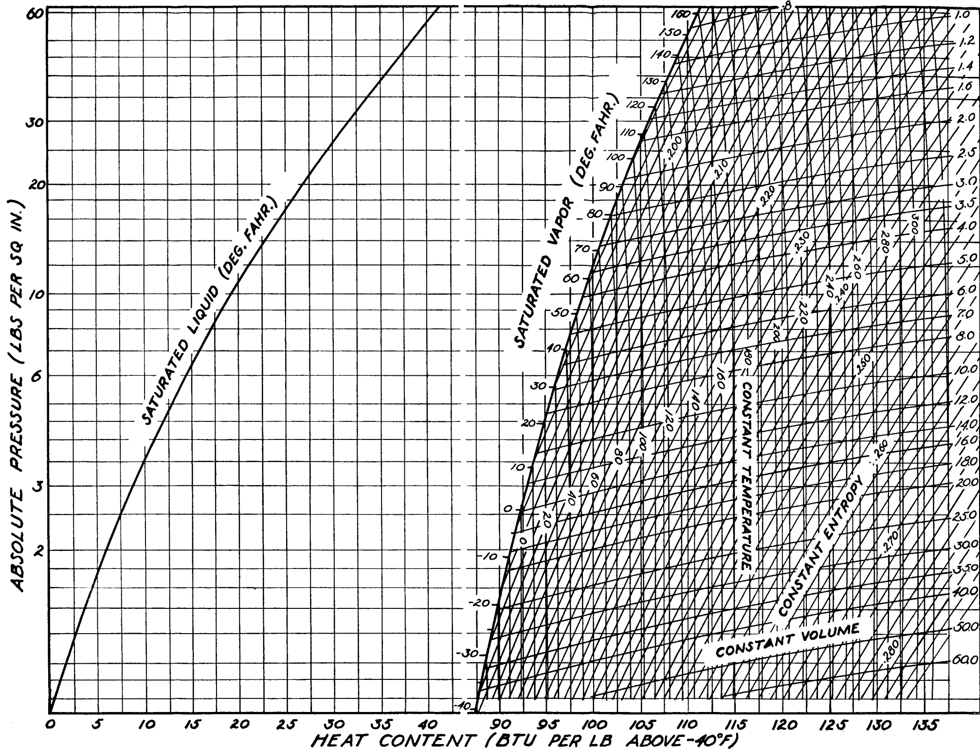
Pressure-Enthalpy Chart for Freon-11. (From Data of Kinetic Chemicals, Inc.)
