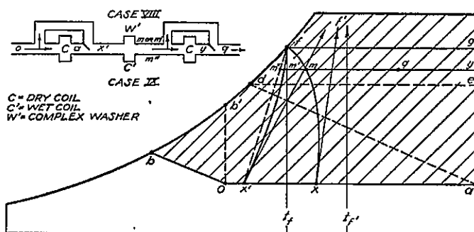
FIG. 12-5. Tempering Coil, Complex Washer (or Wet Surface), and Reheat Coil.
