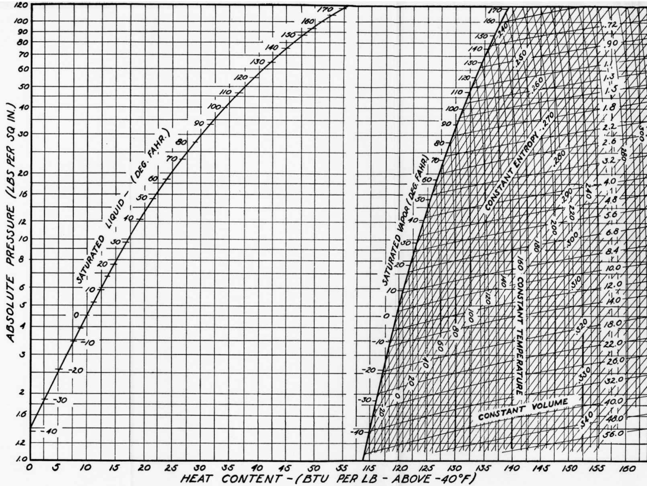
Pressure-Enthalpy Chart for Freon-21. (From data of Kinetic Chemicals, Inc.)
