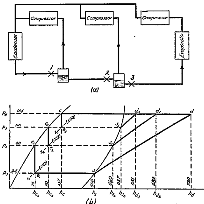
FIG. 3-2. Sectionalized Compression with Multiple Expansion Valves.
