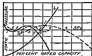
FIG. 15-9. Parallel Operation of Fans.
