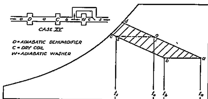
FIG. 12-11. The Over-dehydration Cycle.
