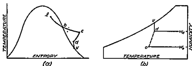
FIG. 11-13. Steam Jet Humidification.
