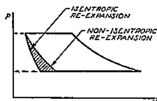
FIG. 2-10. Polytropic Re-expansion.
