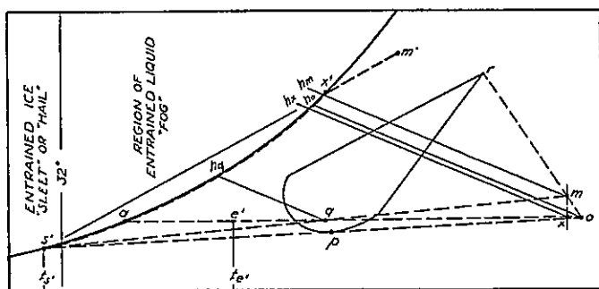
FIG. 11.7. Dehumidifying Coil Performance.
