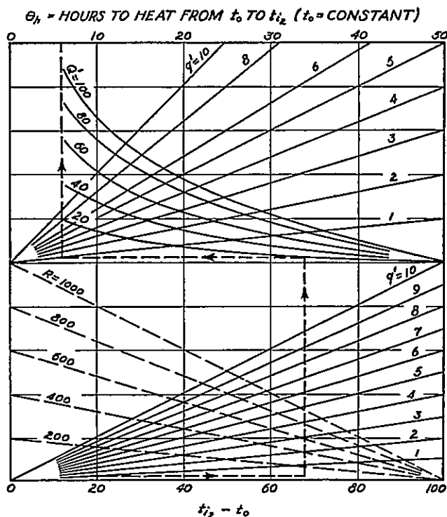
Fig. 8-2. Graphical Solution of Heating Equation.
