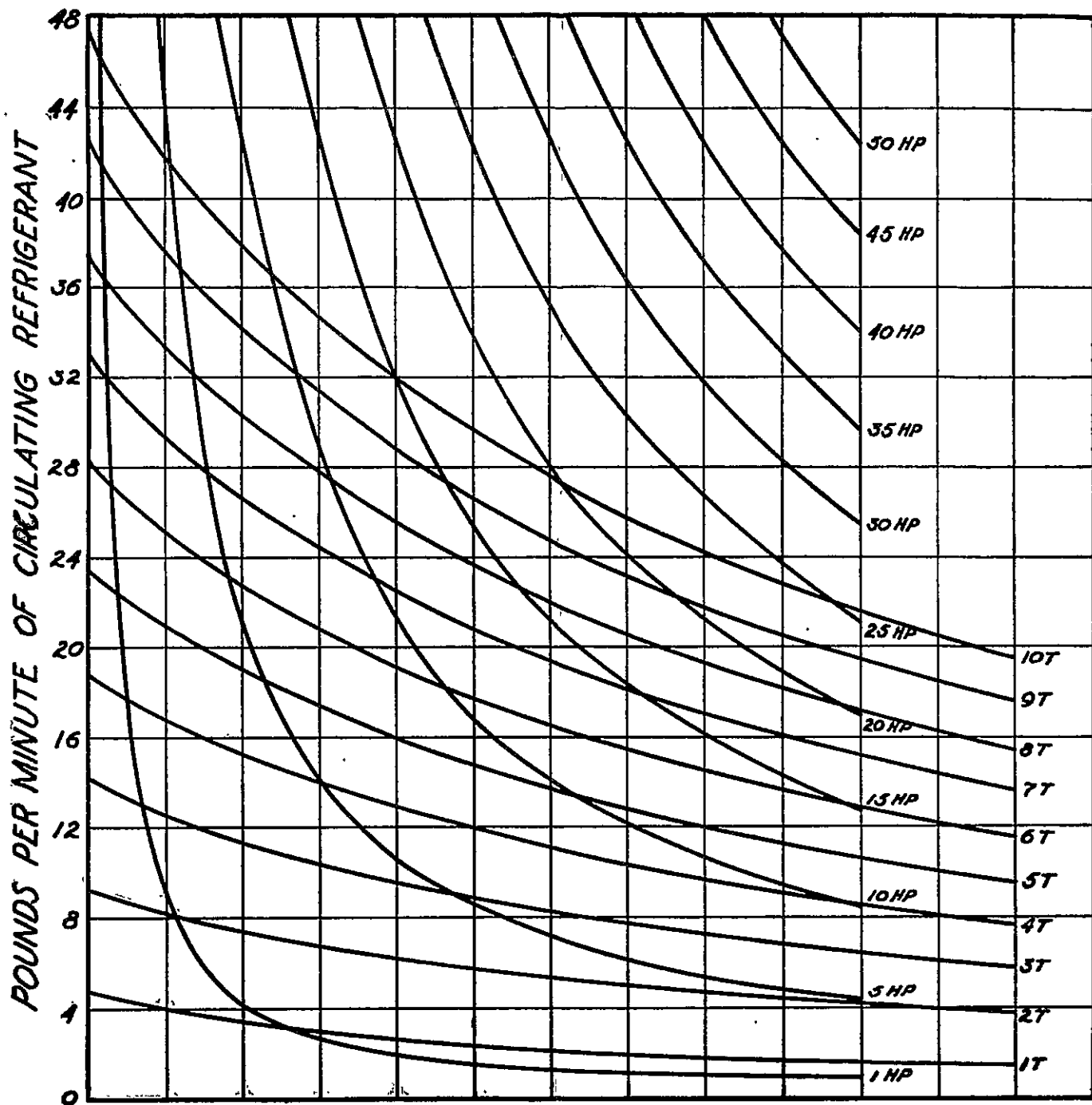
Trace Sheet for Freon-11:
