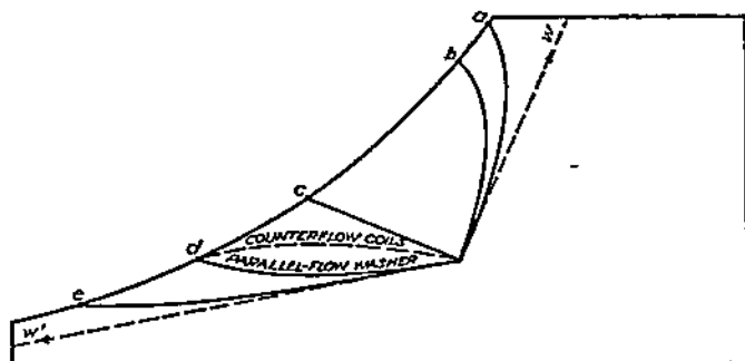
FIG. 11-15. Washer Processes: Low Water-air Ratio.
