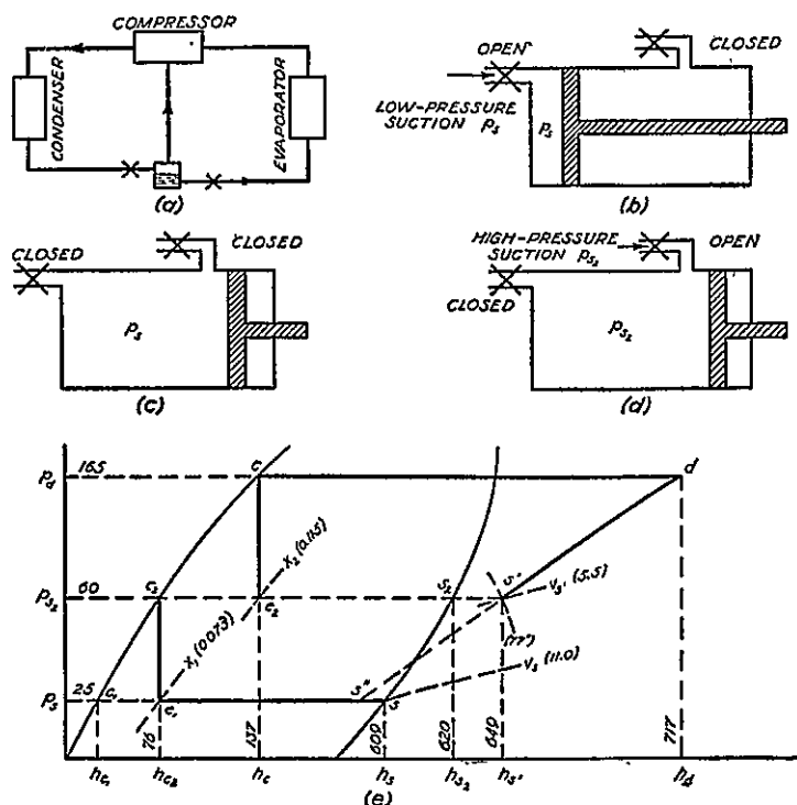
FIG. 3-6. Dual-effect Compression.
