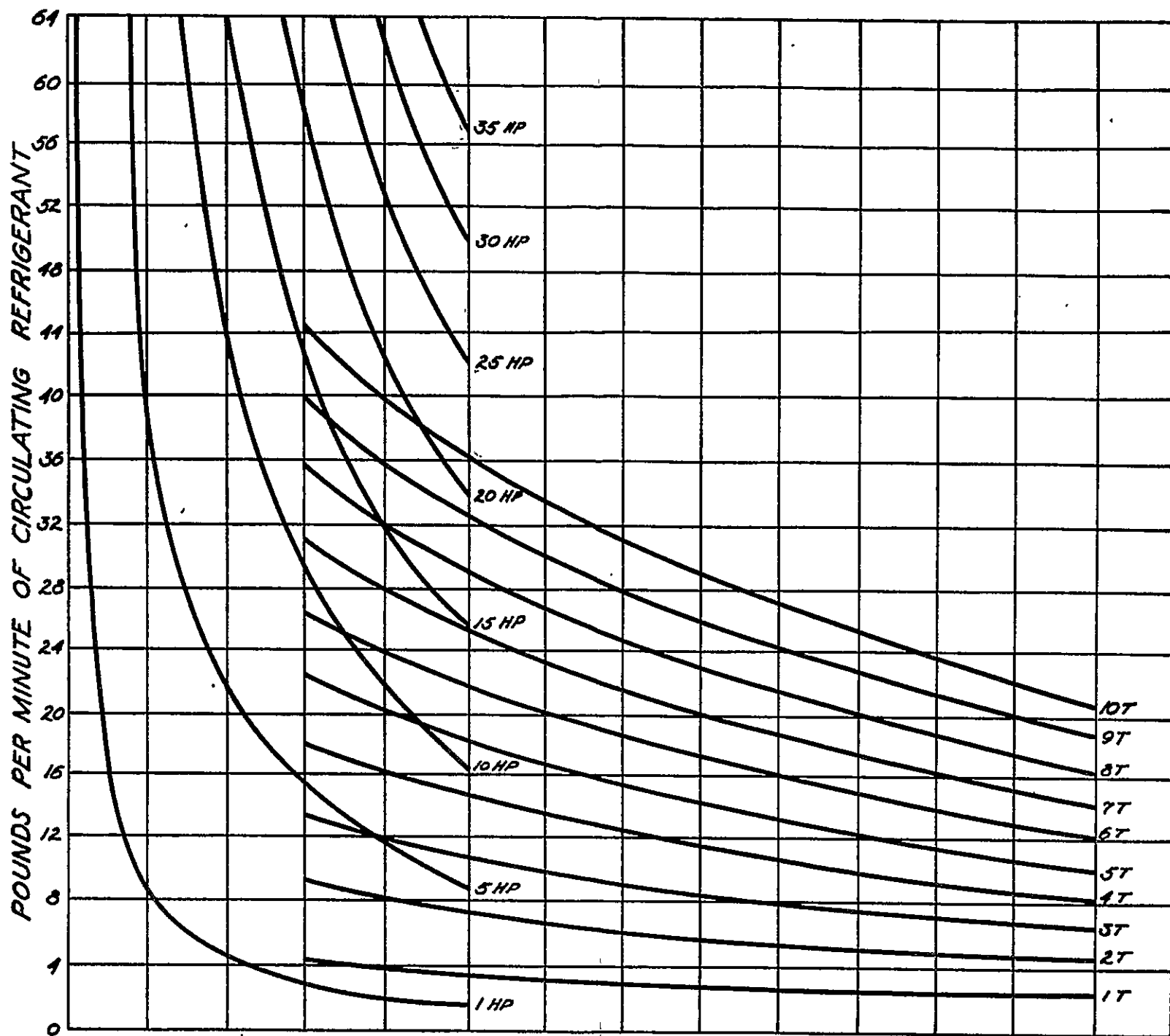
Trace Sheet for Freon-12.
