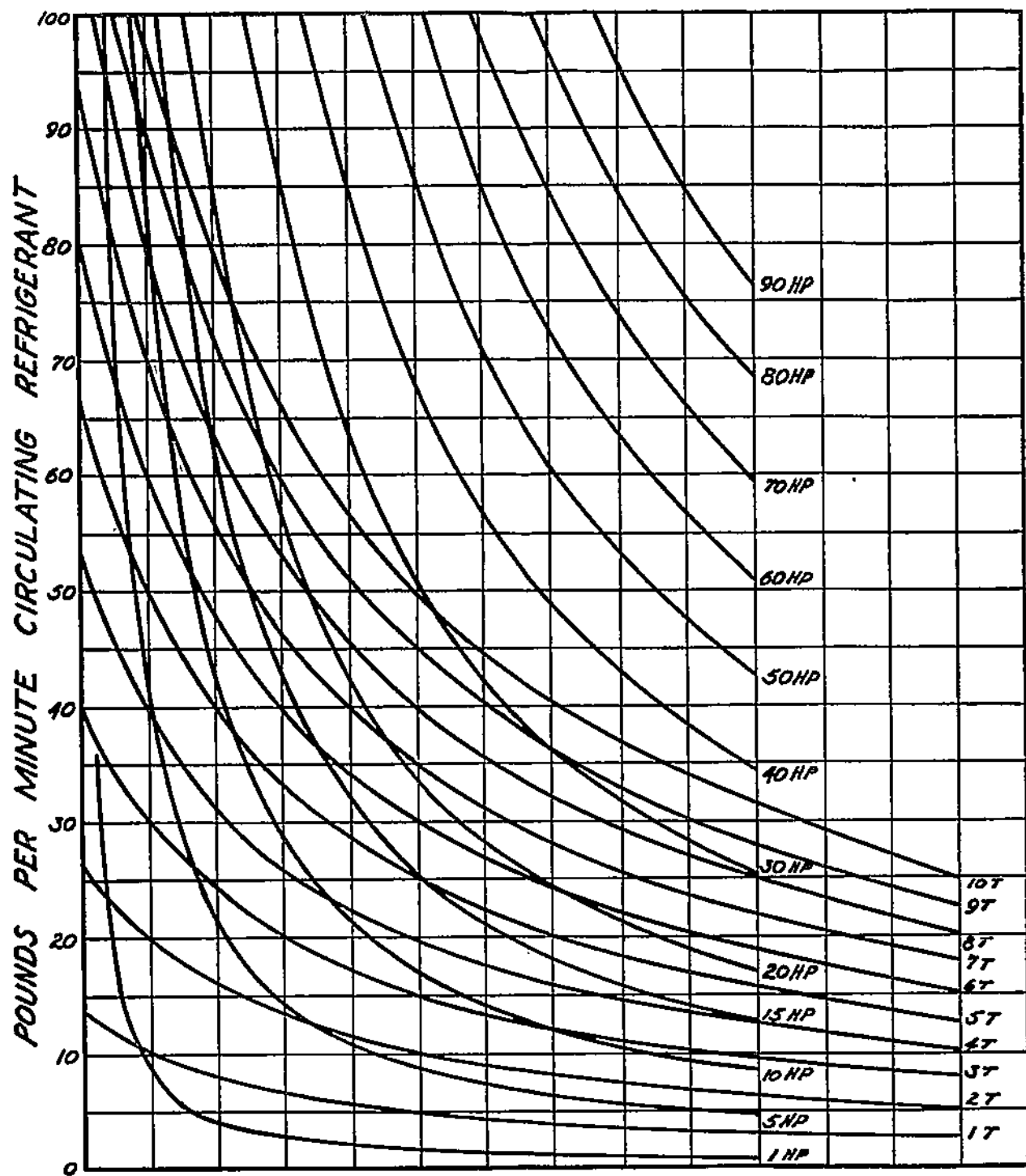
Trace Sheet for Freon-113.
