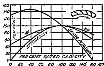
FIG. 15-4. Backward Blade Characteristics.
