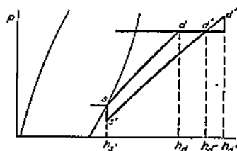
FIG. 4-5. Power Losses from Wire-drawing.
