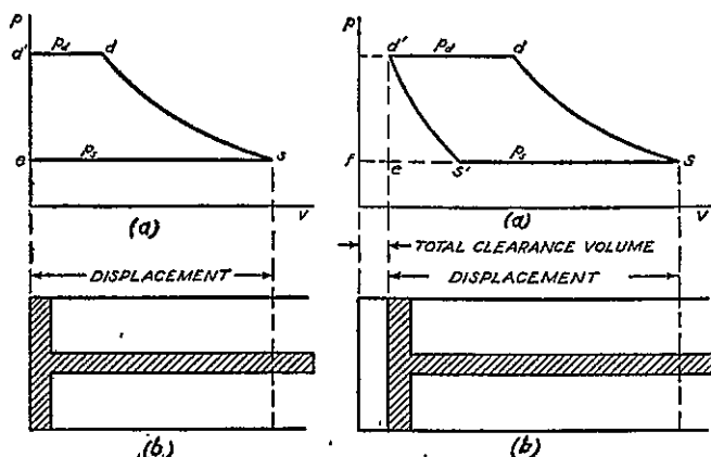
FIG. 2-8. Zero Clearance.
