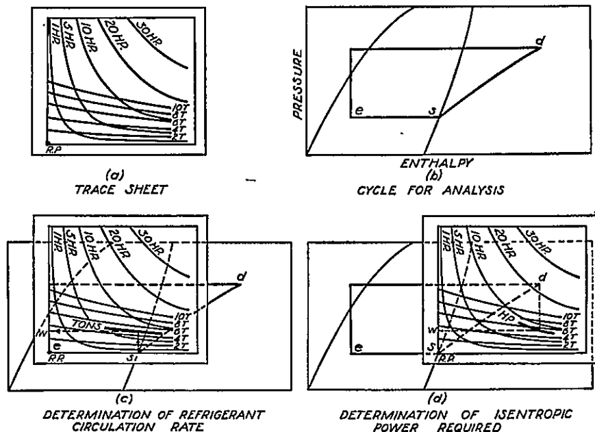
FIG. 3-15. Graphical Solution of Cycle by Use of ph Chart and Trace Sheet.
