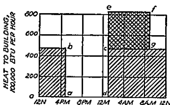
Fig. 8-5. Typical Time-Load Relationship.
