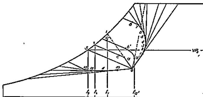
FIG. 11-12. Spray Dehumidification Processes.
