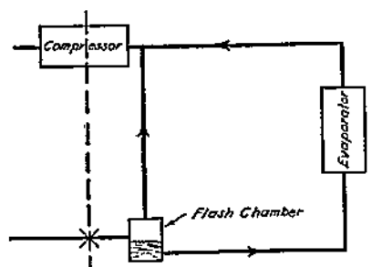
Fig. 2-2. Evaporator with Flash Chamber.
