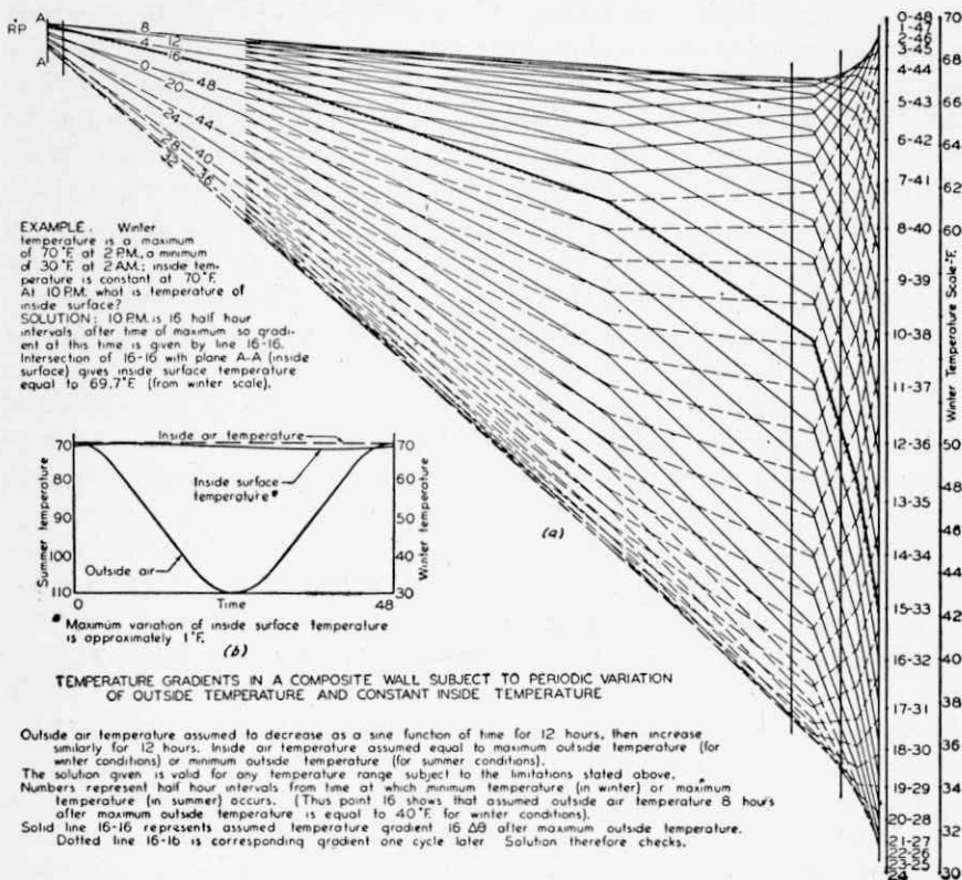
FIG. 7.7. Graphical Solution of Composite Wall Problem.
