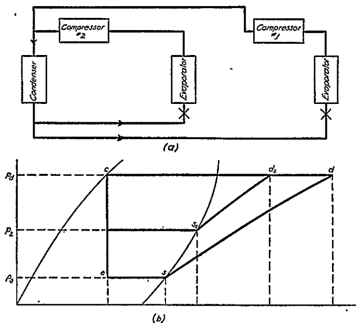
FIG. 3-9. Parallel Operation:
