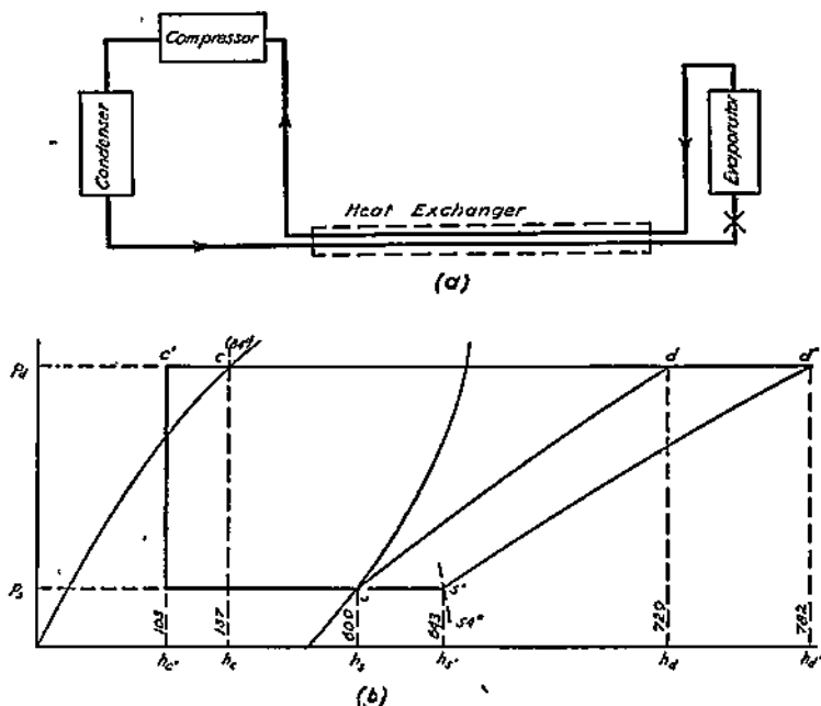
FIG. 2-6. Subcooling with Vapor.
