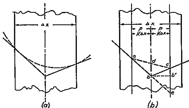
FIG. 7-1. Method of Finite Differences
