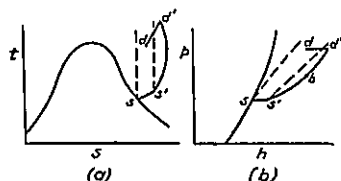
FIG. 4-4. Heat Transfer throughout Compression.
