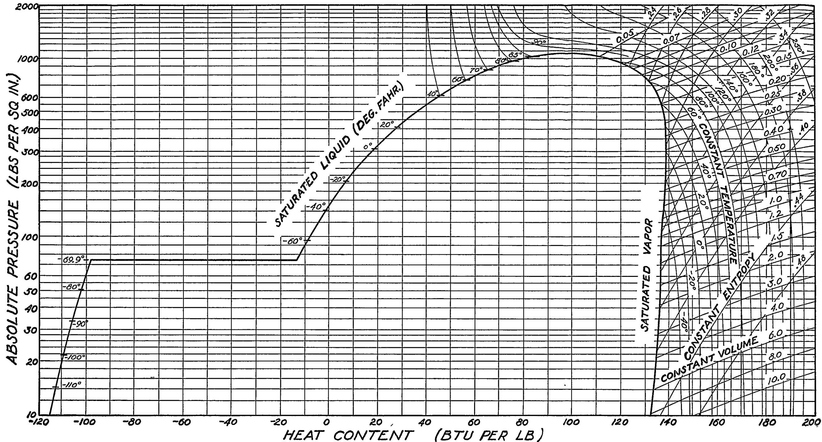
Pressure-Enthalpy Chart for Carbon Dioxide. (From data published by ASRE.)
