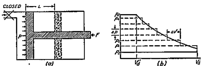
FIG. 1-2. Work during Expansion or Compression.
