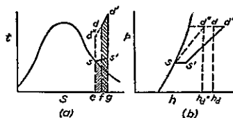
FIG. 4-2. Heat Transfer during Admission and Discharge.
