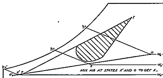
FIG. 10-5. Straight Line (Approximate) Mixing.
