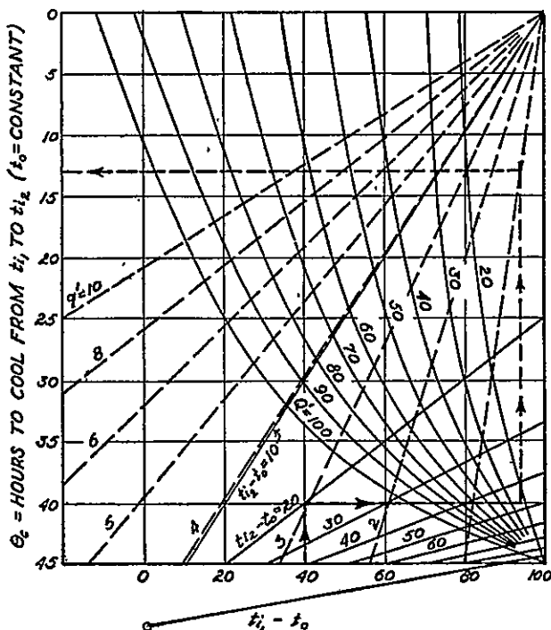
FIG. 8-1. Graphical Solution of Cooling Equation.
