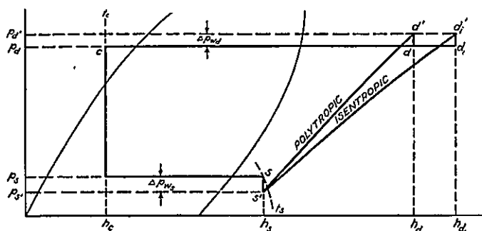
FIG. 4-1. Throttling Losses at Suction Discharge Valves:
