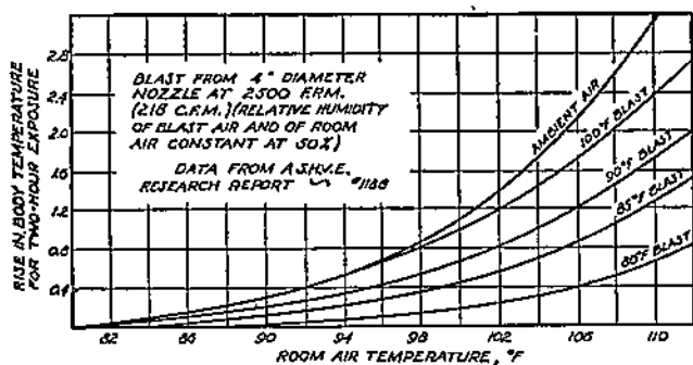
Fig. 14-3. Local Cooling by Air Blast:
