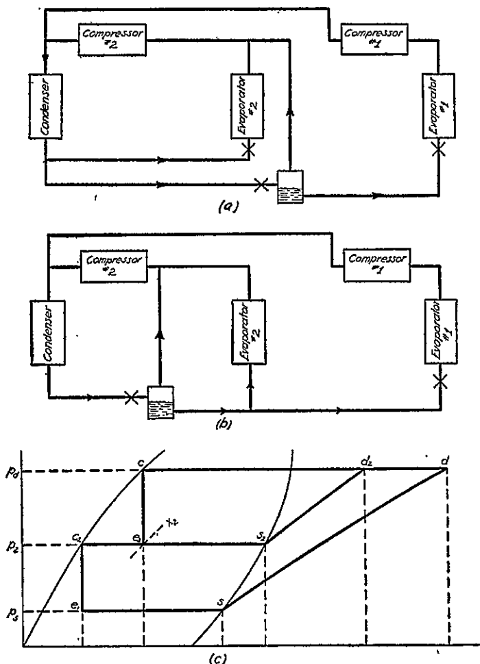
FIG. 3-10. Sectionalizing.
