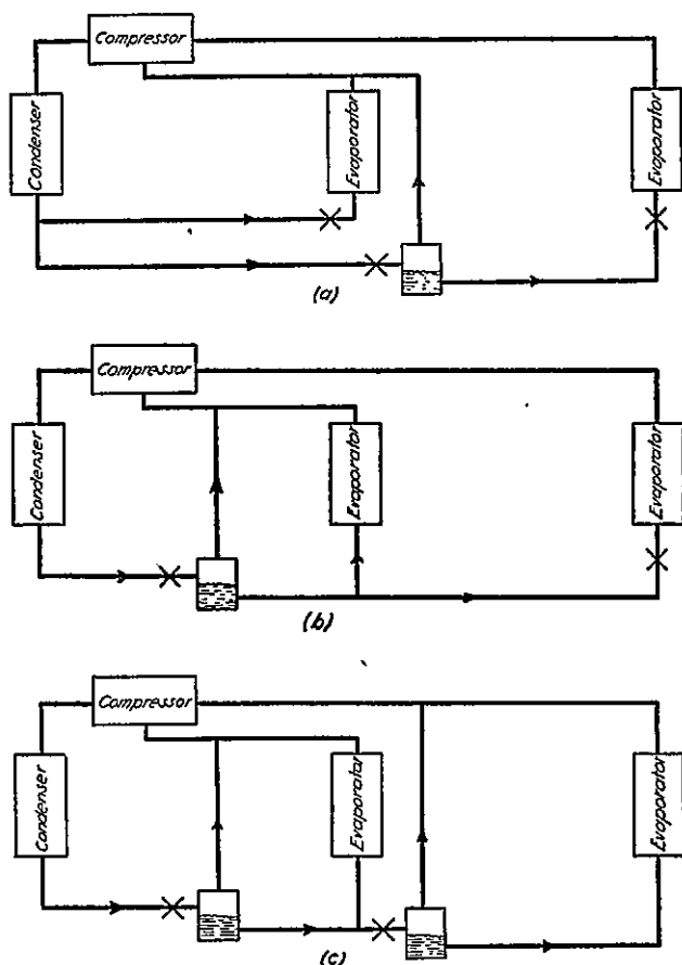
FIG. 3-13. Alternate Multi-effect Arrangement (Thermodynamically Idealized).
