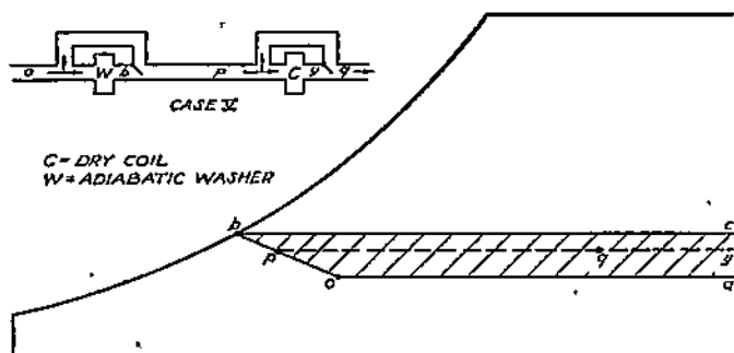
FIG. 12-2. Adiabatic Washer and Reheat Coil.
