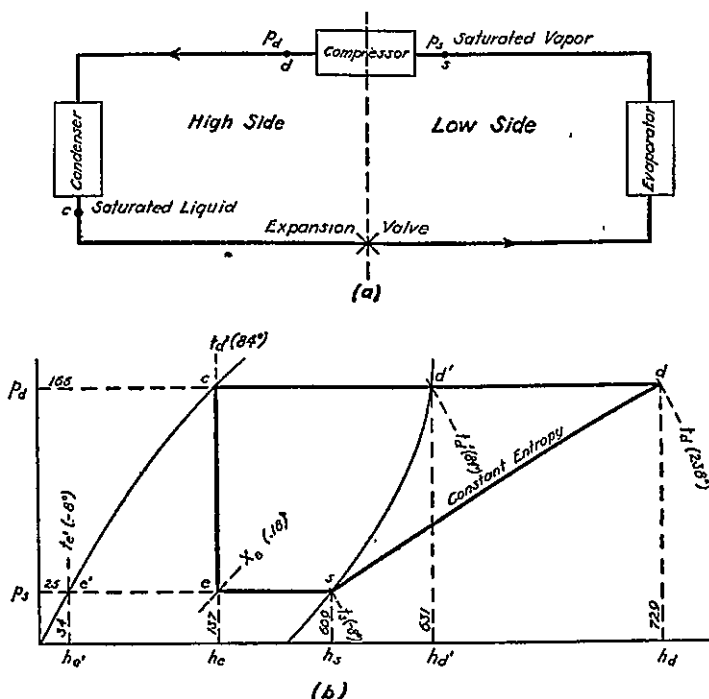
FIG. 2-1. Simple Saturation Cycle.
