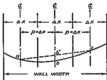
Fig. 7-2. Construction for K = 1 .
