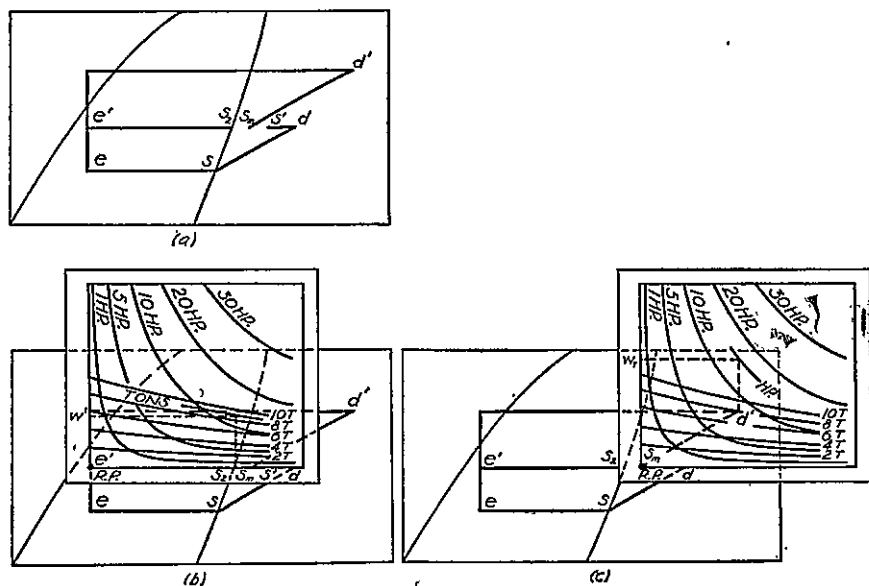
FIG. 3-17. Twin-load Cycle Analysis.
