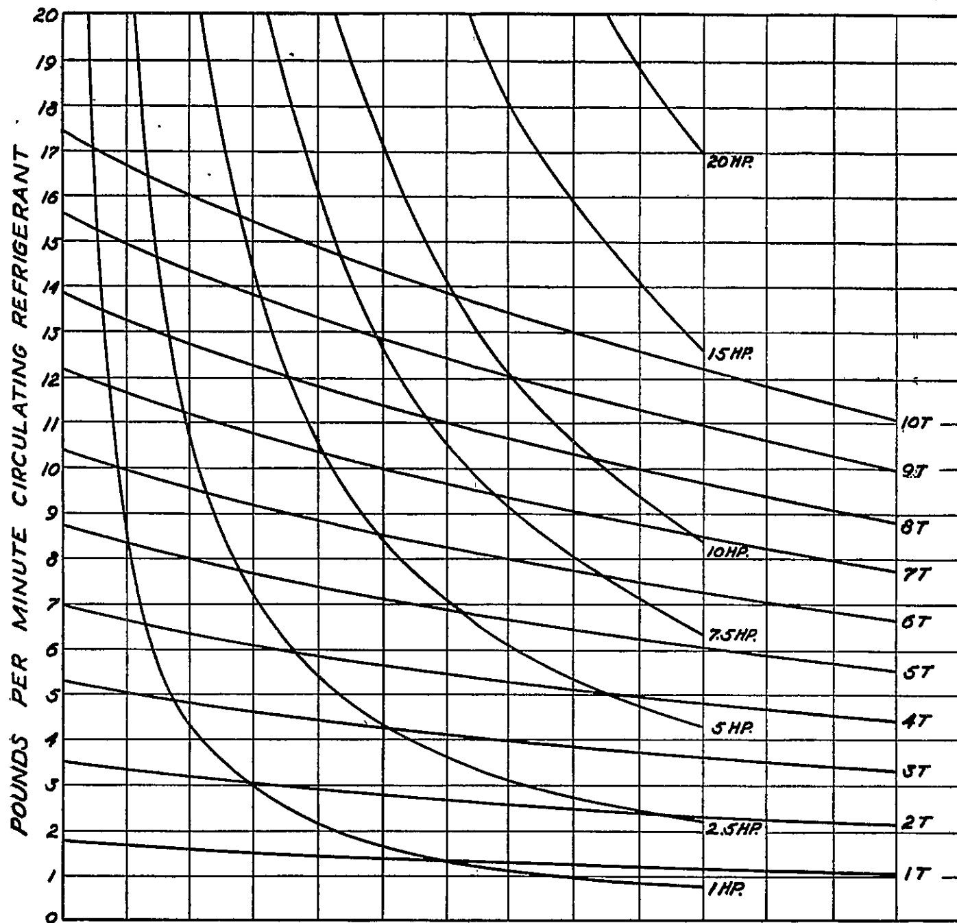
Trace Sheet for Methyl Chloride.
