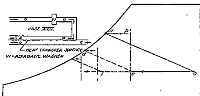
FIG. 12-13: Indirect Evaporative Cooling.
