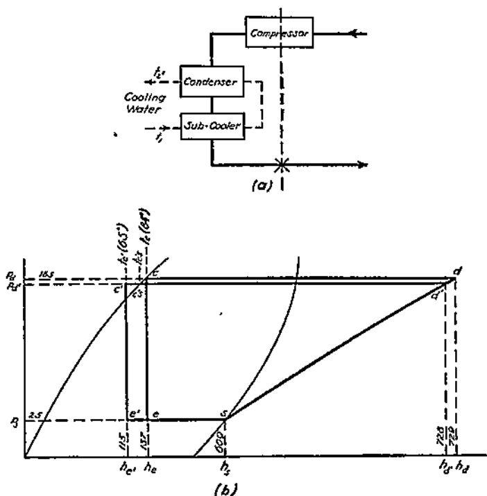
FIG. 2-4. Saturation versus Subcooling Cycle.
