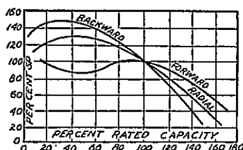
Fig. 15-7. Comparative Static Pressure Curves.
