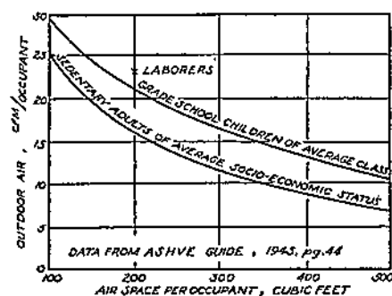
FIG. 13-1. Outside Air Ventilation Requirement for Odor Control.
