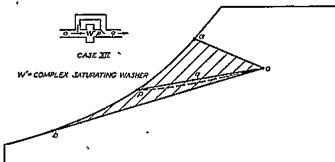
FIG. 12-8. Cooling by Complex Saturating Air Washer.
