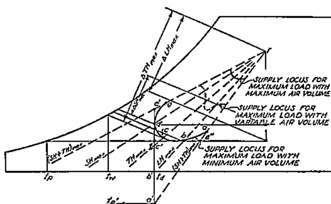
Fig. 10-2. Five Critical Loading Conditions.
