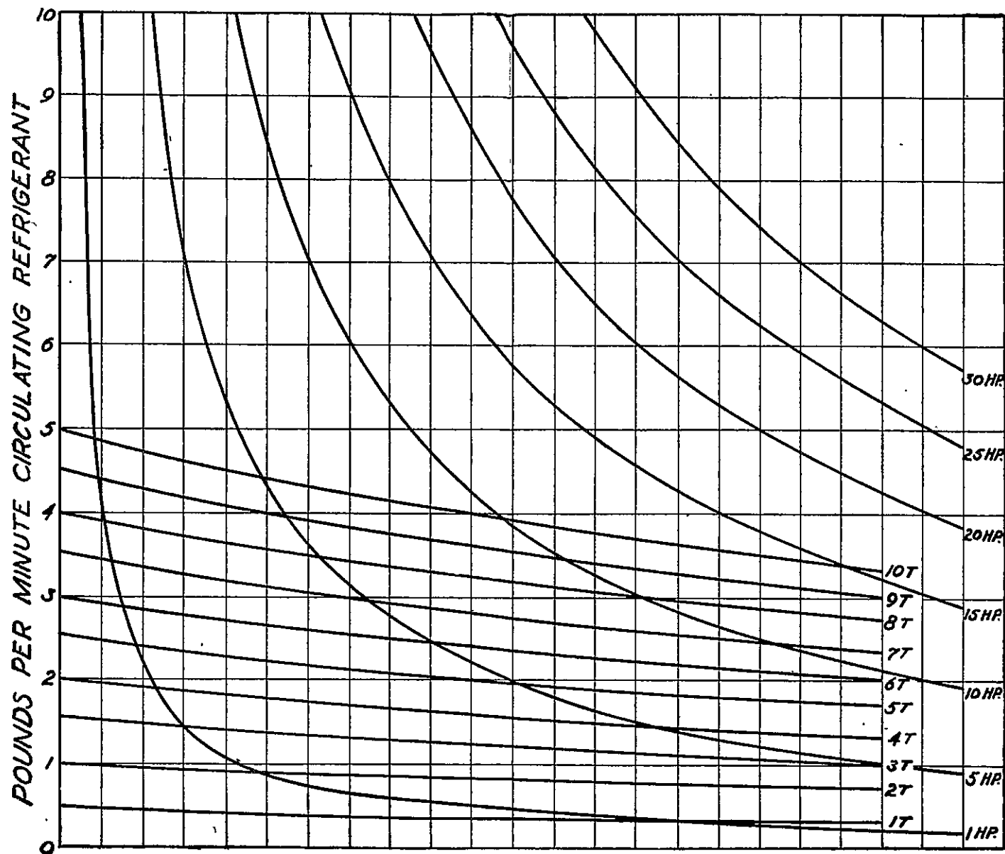
Trace Sheet for Ammonia.
