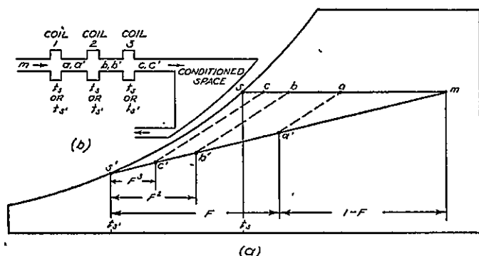
Fig. 11.8. Constant-temperature Coils in Series.
