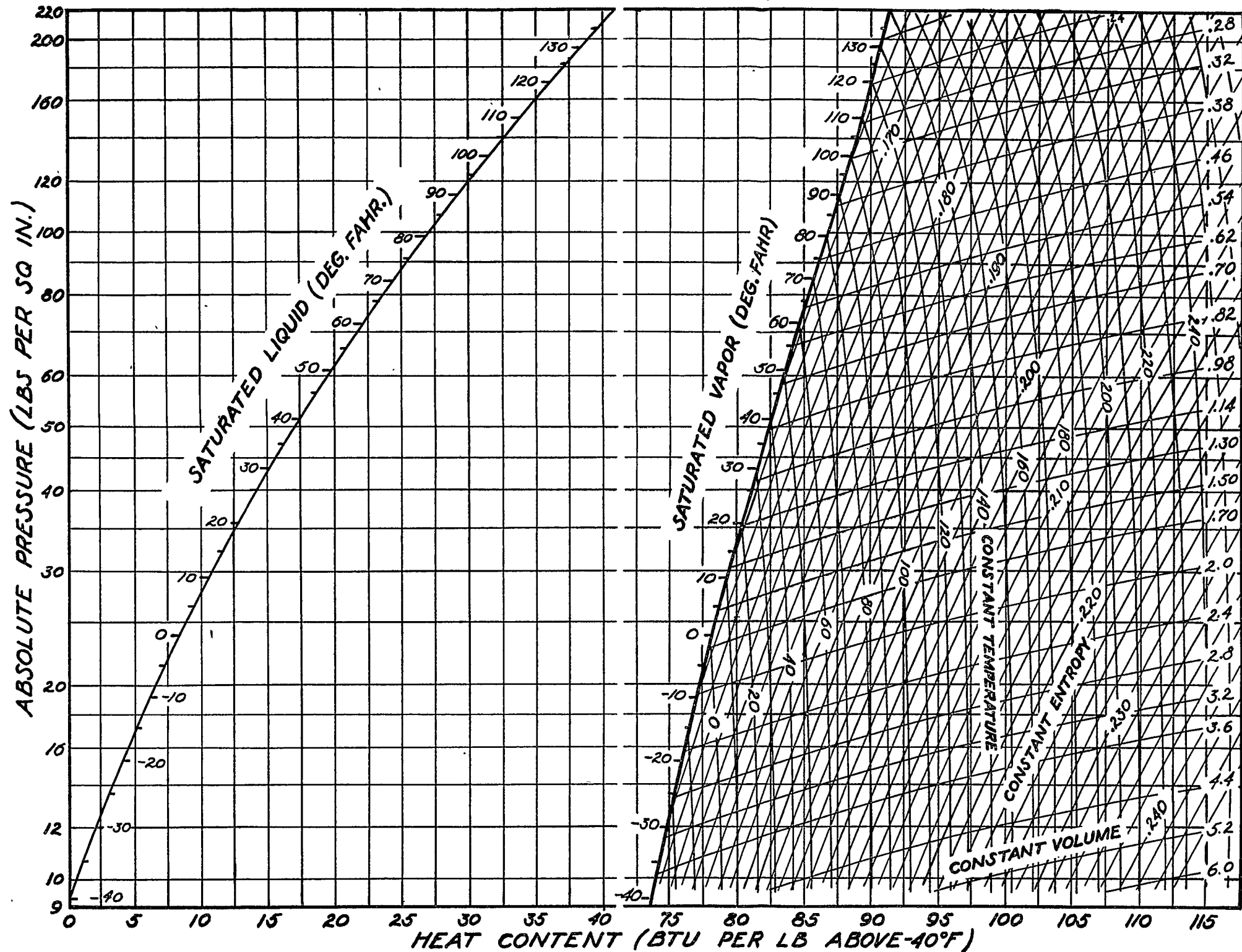
Pressure-Enthalpy Chart for Freon-12. (From data of Kinetic Chemicals, Inc.)
