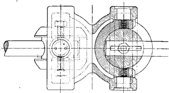
FIG. 78. — Joint Goubet.
